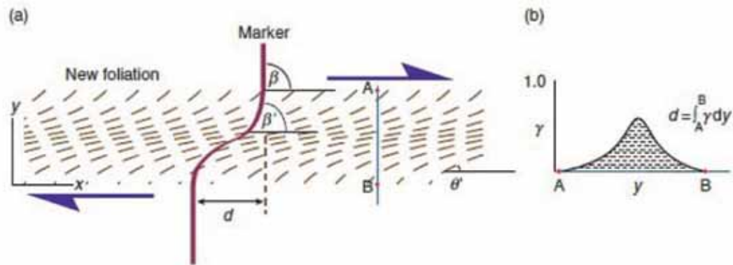
Figure 10. (a) Shear zone with genetically related foliation. The foliation makes 45^{\circ} with the shear zone along the margins. This angle is reduced as strain increases toward the centre of the zone. \beta^{\circ} is the angle between the shear zone and the foliation, (b) The displacement can be found by measuring or calculating the area under a shear strain profile across the zone if the deformation is simple shear (source: Fossen, 2010).
