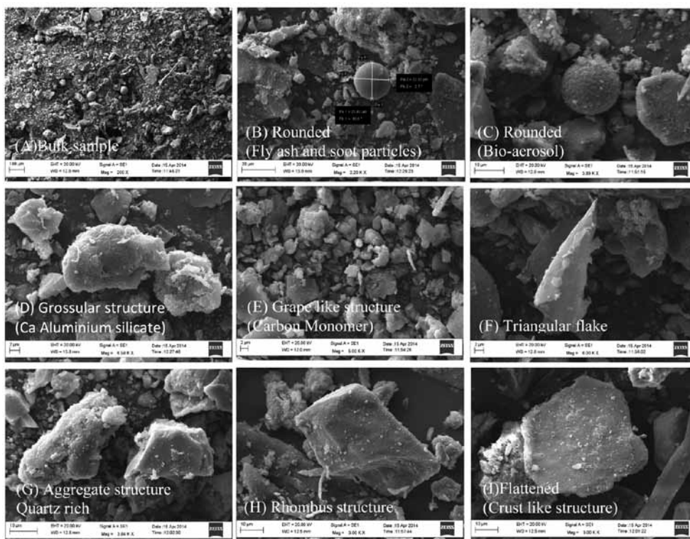
Figure 3. (A to I) SEM Images of dust particles with different magnifications.
