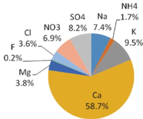
Figure 2. Relative percentage contribution of major ions in dustfall.
