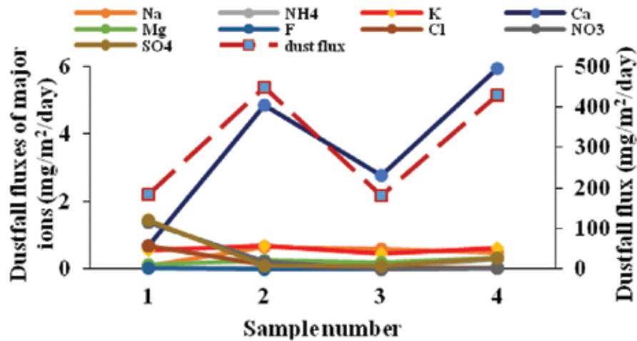
Figure 1. Variation of dust fall flux and major ion fluxes from Nov.2013 to Feb. 2014.
