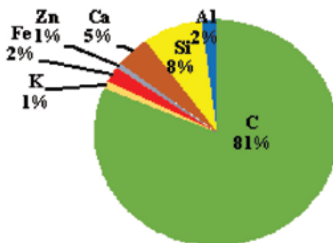
Figure 4. Average elemental composition of dust sample (excluding oxygen %).
